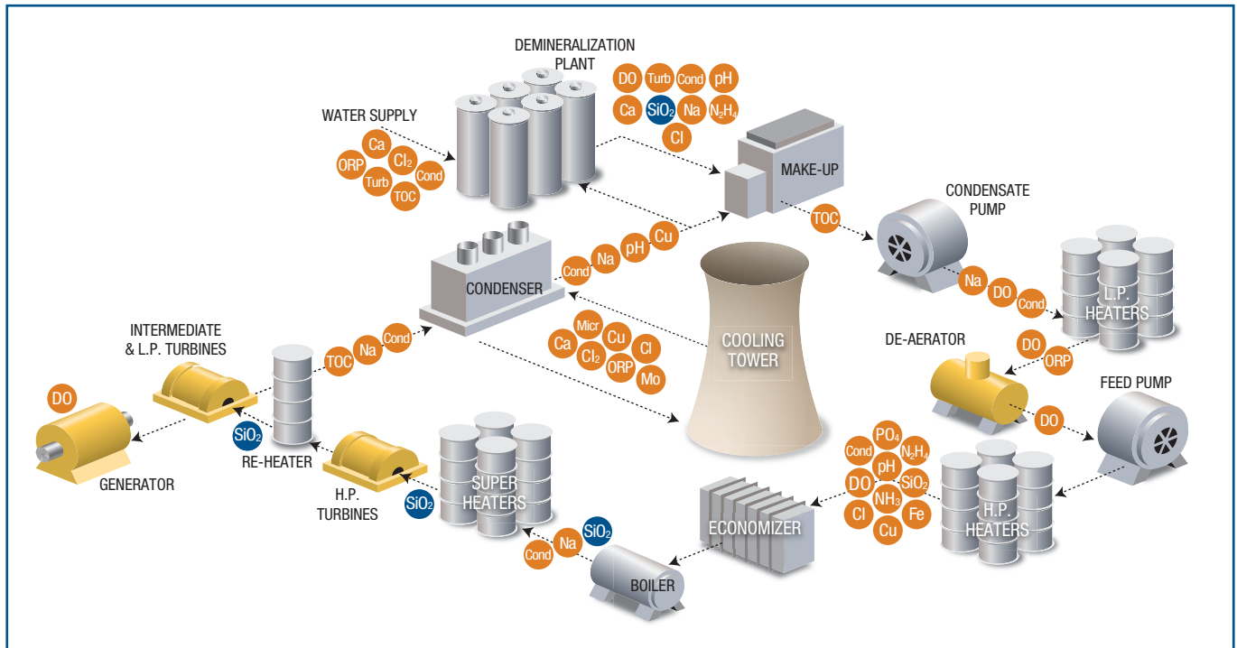
Silica measurement locations in a power plant
