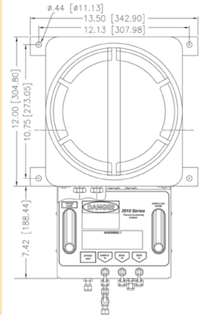
2010 Depth=8.41[213.54]
